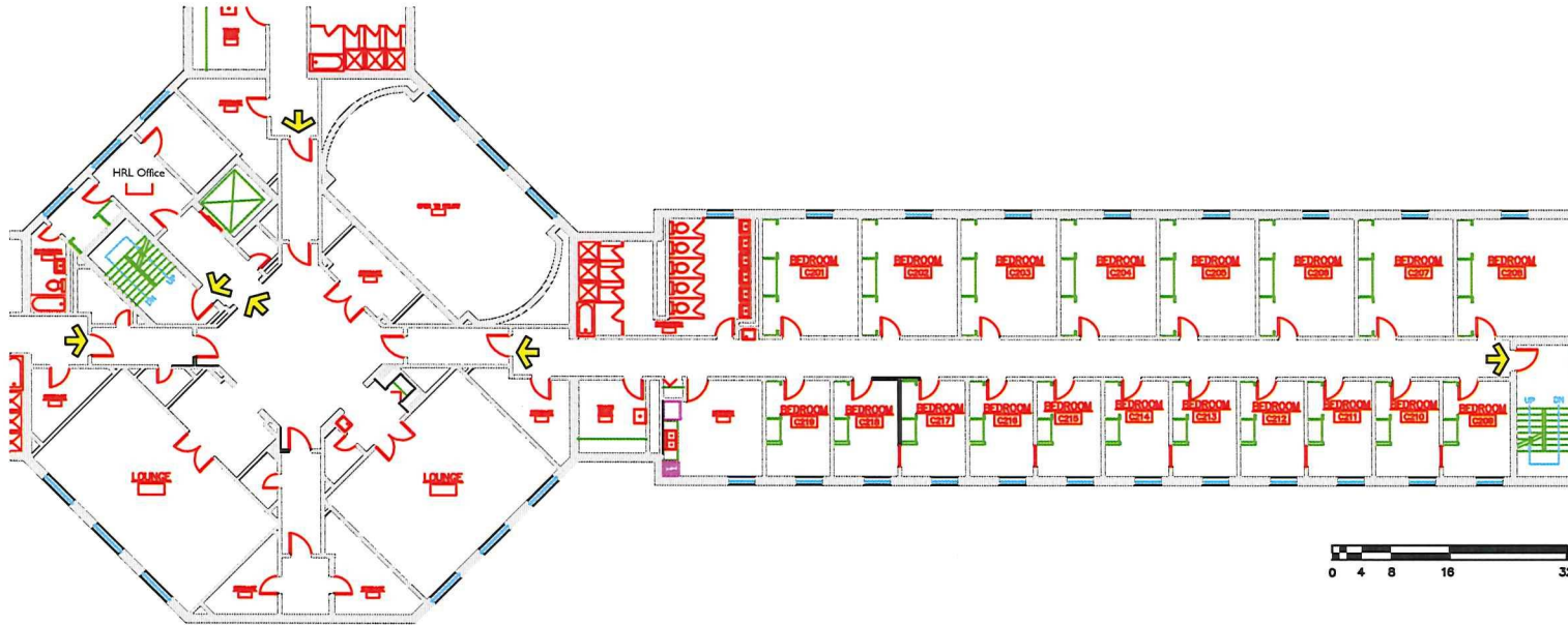
Wing C Second Floor Tinker House Hollins University
