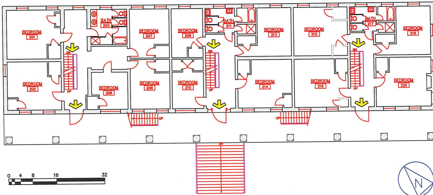
Second Floor Plan East Building Hollins University
