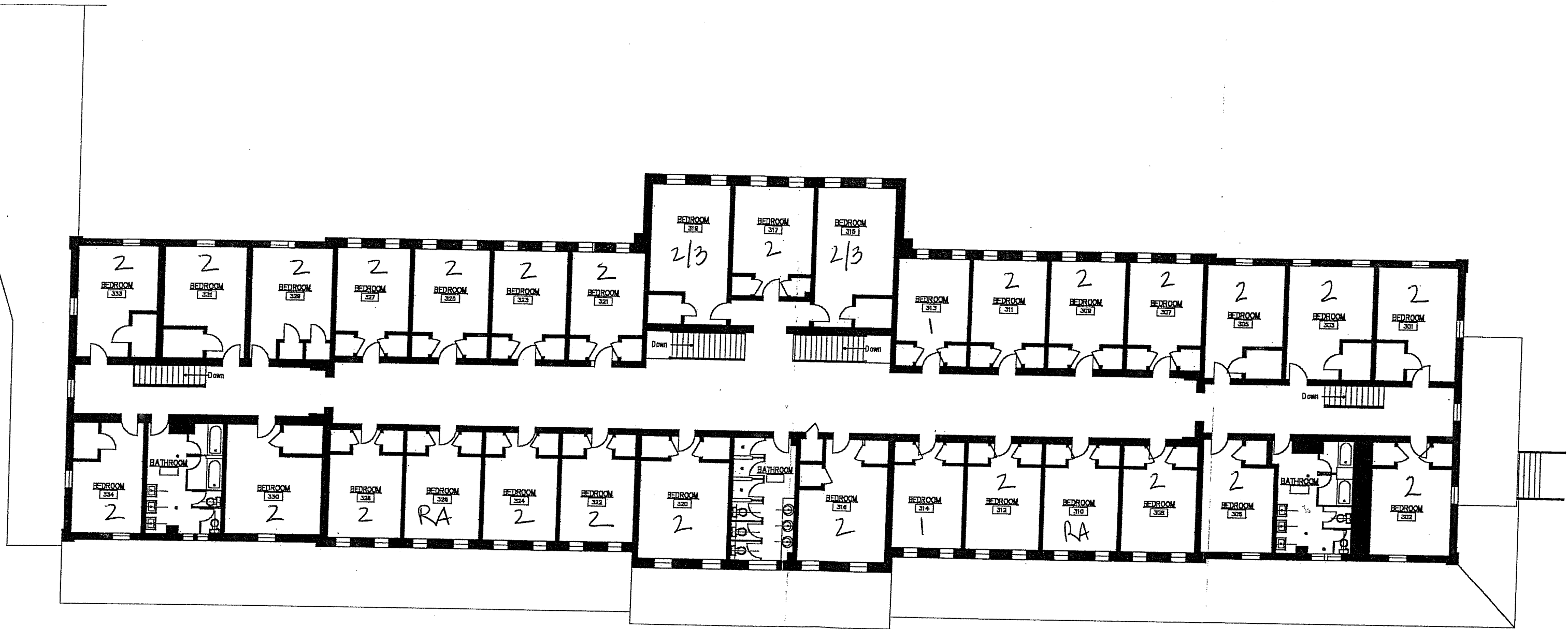
Third Floor Plan West Hall Hollins University
